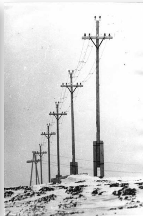
A single-circuit 10 kV electrical line with a reduced phase to-phase distance.
